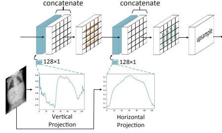
Fig. 4. The architecture of OSE layer.
